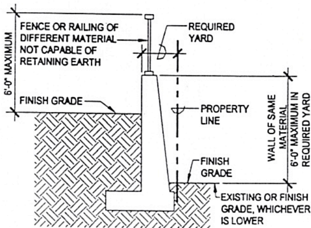
RETAINING WALLS WITH SAFETY RAILINGS
