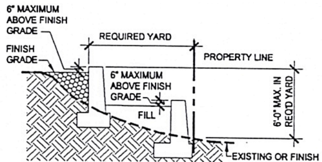
TERRACED RETAINING WALLS
