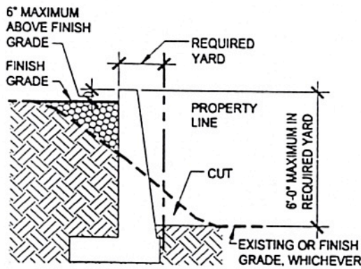
CUT and FILL RETAINING WALL
